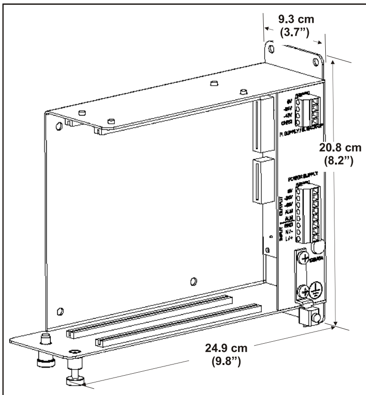
Figure 1: Wall-Mount Chassis
