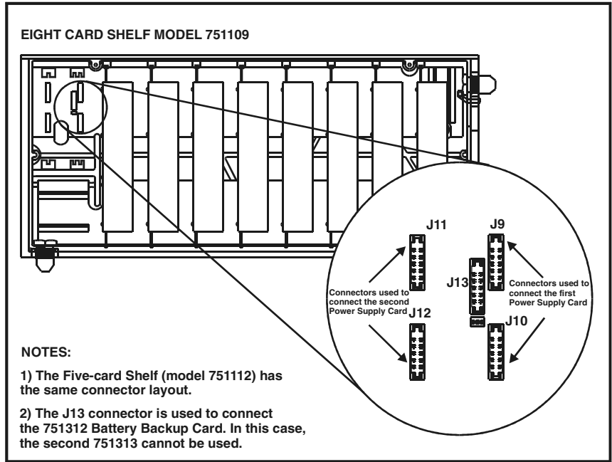
Figure 3 Model 751313 Installation Location
