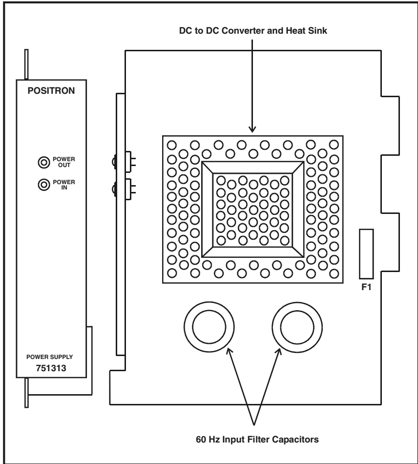
Figure 1 Model 751313 Component Layout
